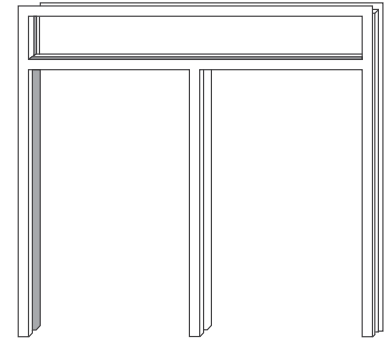
SIDE MULLION & TRANSOM
