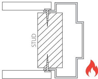
PARTITION
