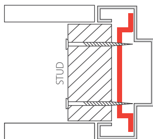
TOP HAT FIXING (FLUSH FINISH WALL)
