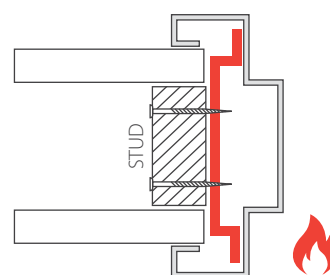
TOP HAT FIXING (CONCEALED EDGE OF WALL)
