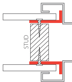
WING STRAP WELDED (CONCEALED EDGE OF WALL)
